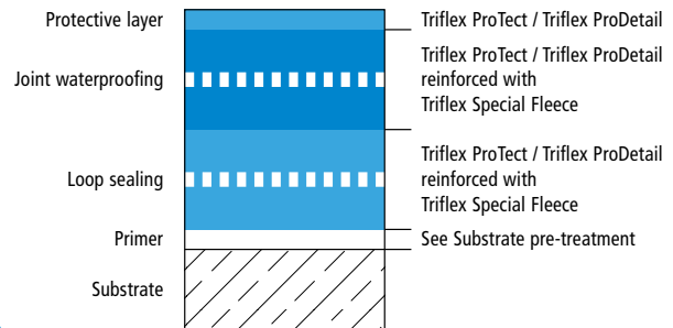
System build-up – Detail B
