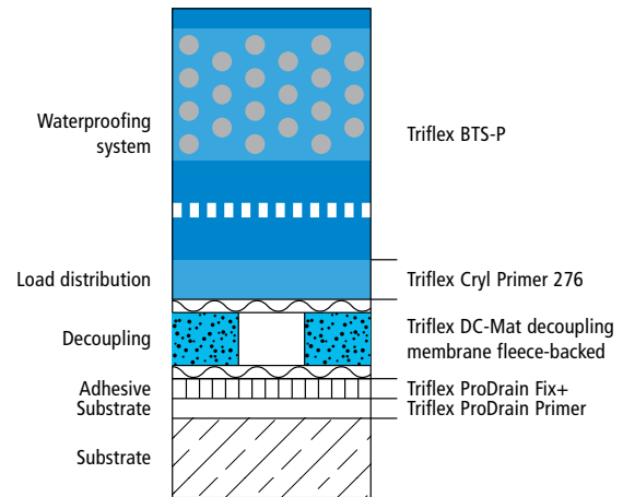
System build-up – Detail A
