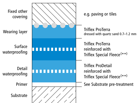
System build-up – Detail B
