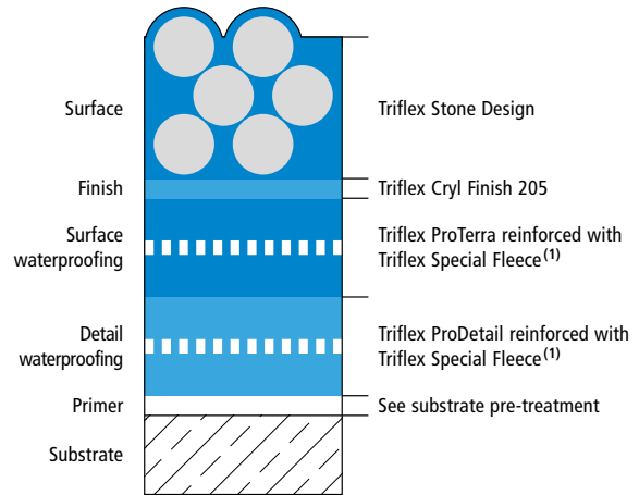
System build-up – Detail
