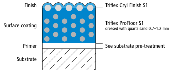
System design, S1 version – Detail B
